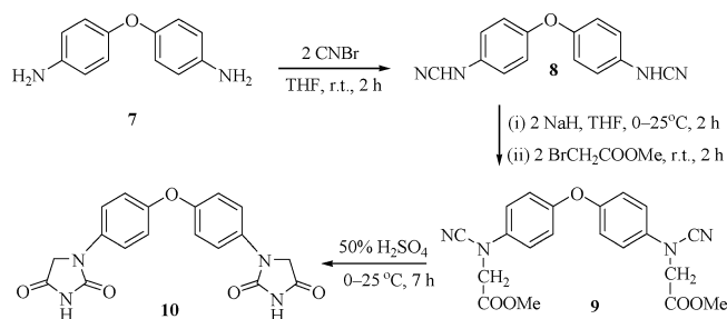
Scheme 3. Synthesis of bis(hydantoin) 10.
