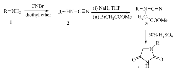
Scheme 1. Synthetic route for N-1 substituted hydantoins.
