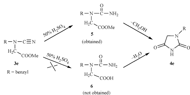
Scheme 2. Mechanism for the formation of 4 from 3 .
